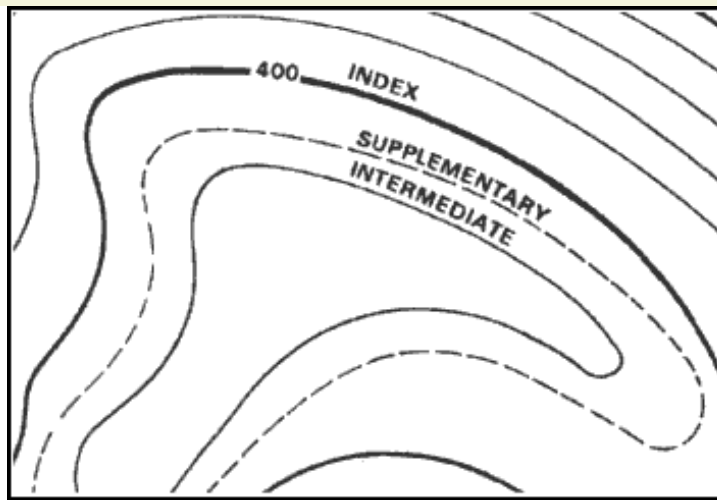
Figure 10-1. Contour lines.
