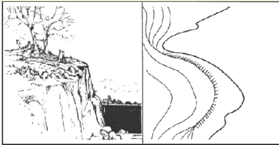
Figure 10-24A. Cliff.
