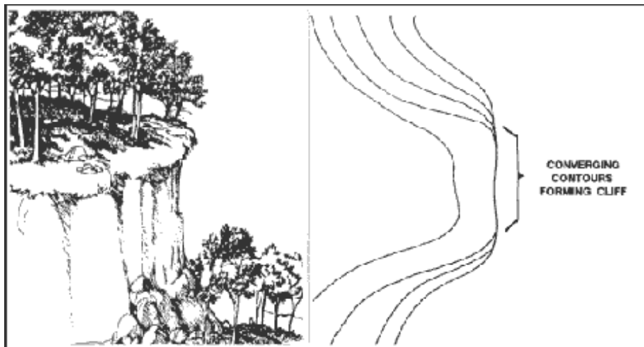
Figure 10-24B. Cliff.
