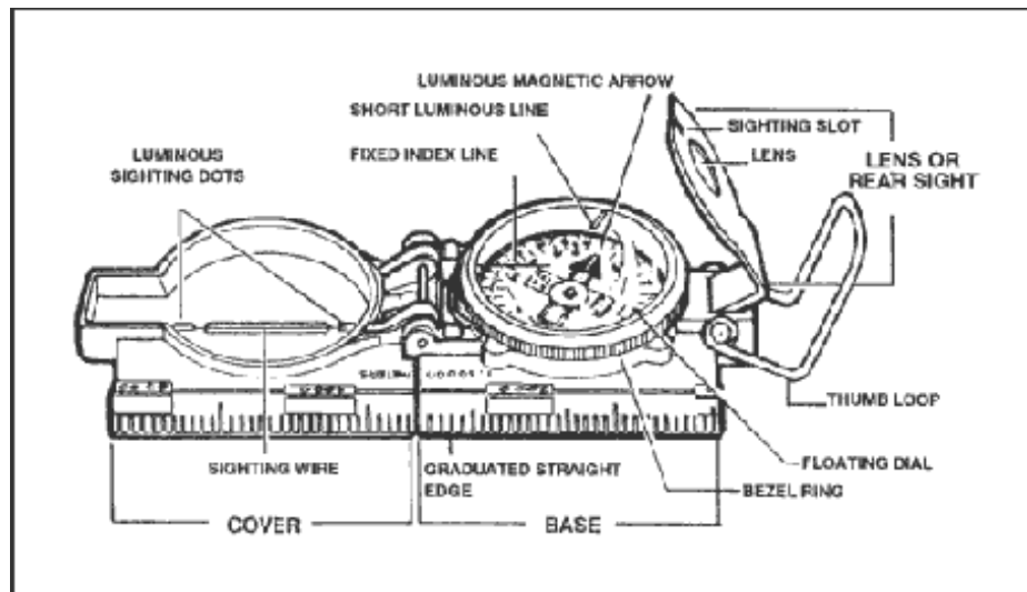
Figure 9-1. Lensatic compass.
