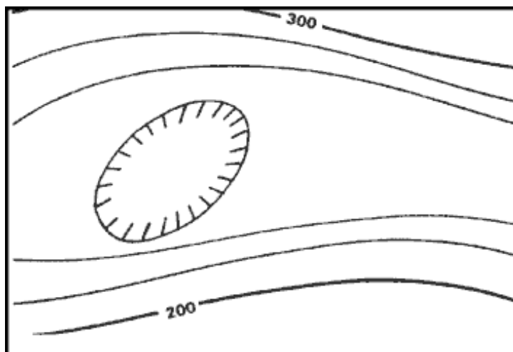
Figure 10-5. Depression.
