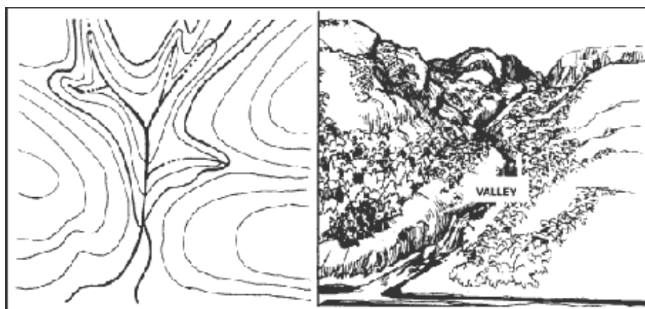
Figure 10-19. Valley.
