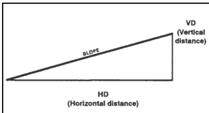
Figure 10-10. Slope diagram.
